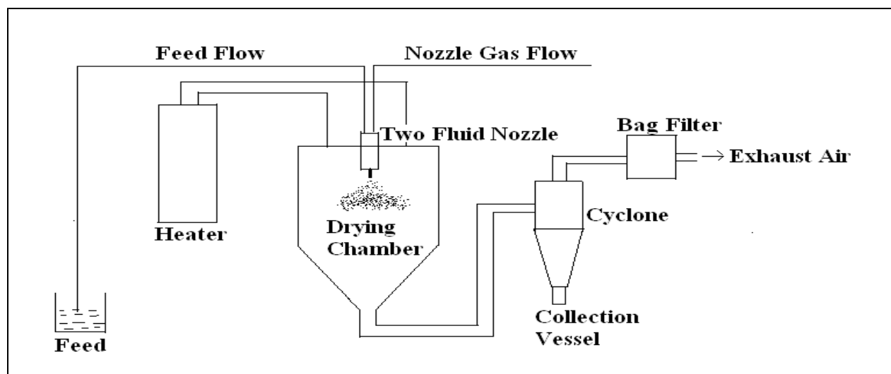
Fig 1 -Spray Drying.
