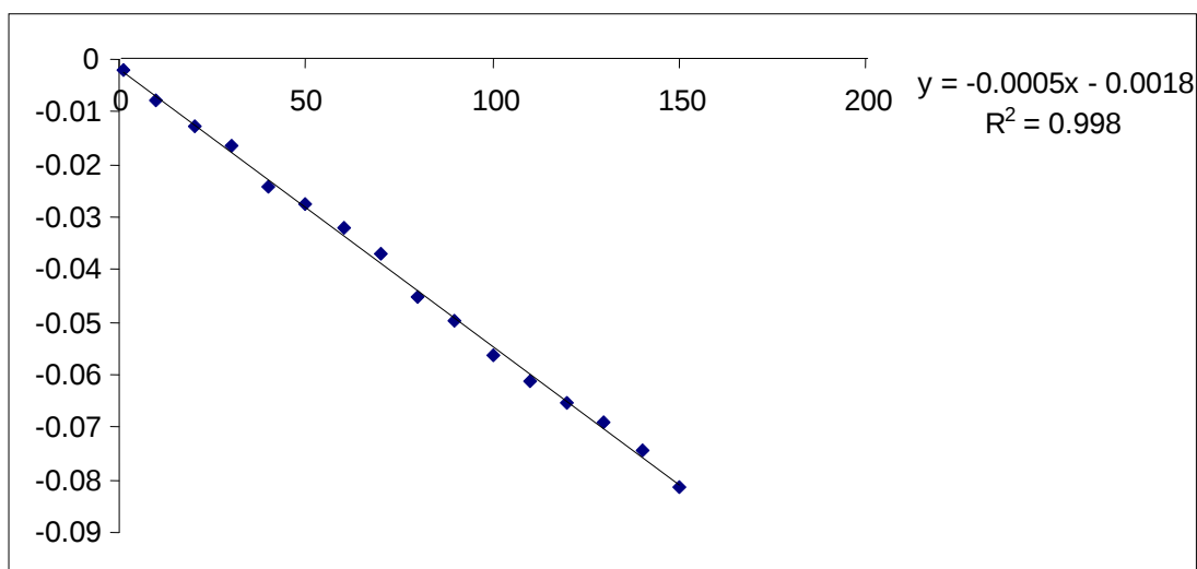
Fig: 5.11. Calibration curve for BDP at 278.5 nm.
