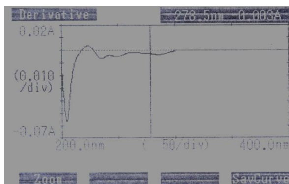
Fig: 5.10. First order derivative spectra of mixture at 278.5 nm.
