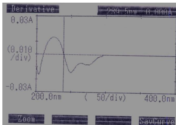
Fig: 5.7. First order derivative spectra of BDP.
