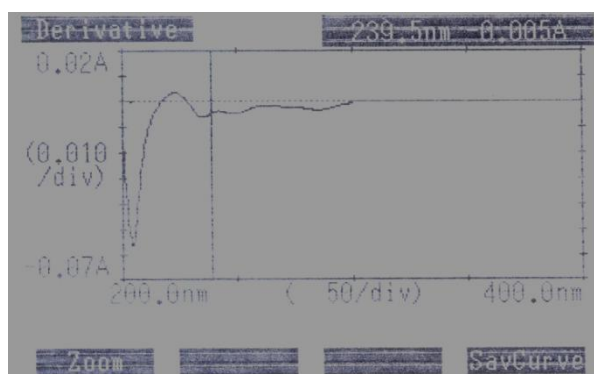
Fig: 5.9. First order derivative spectra of mixture at 239.5 nm.
