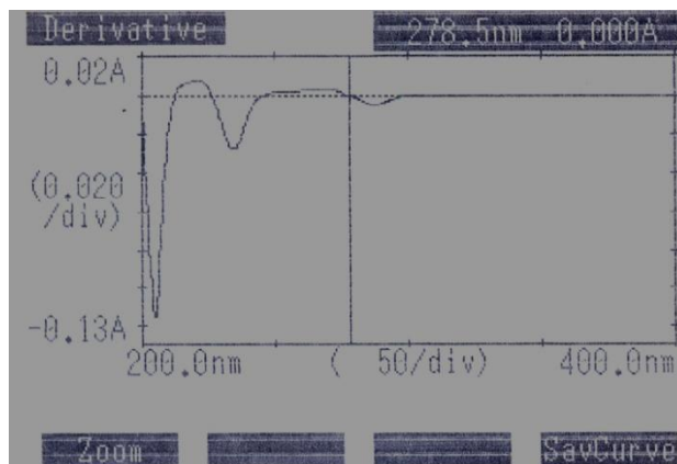
Fig: 5.8. First order derivative spectra of SS.
