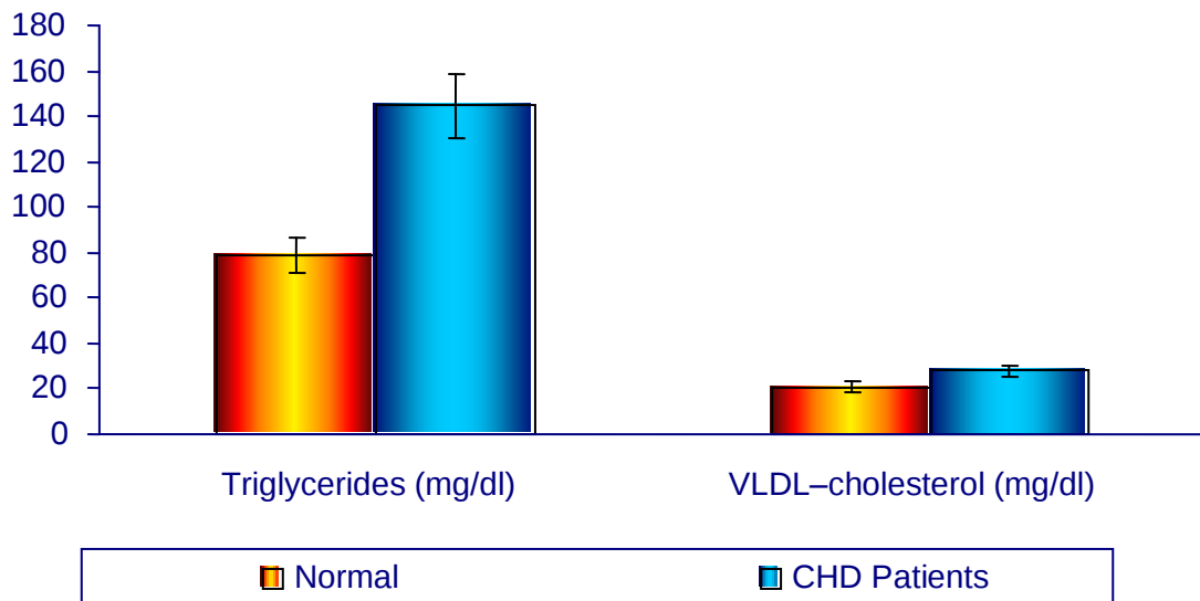
Fig.2: Levels of Triglyceride and VLDL-cholesterol in Normal and CHD Patients
